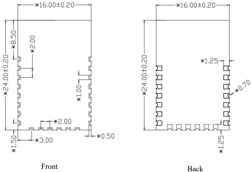
Figure 4 Module size diagram
