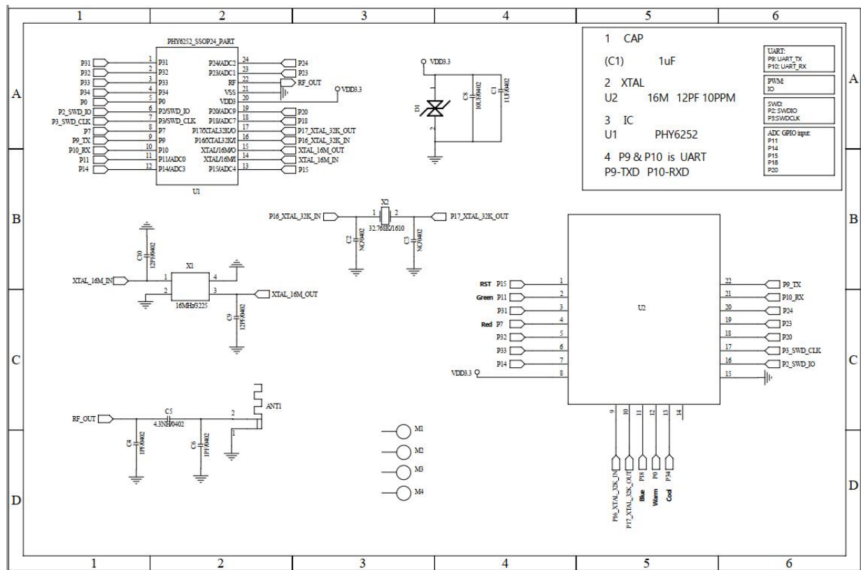
Figure 6 Module schematic
