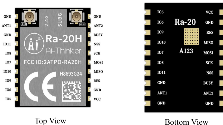
Figure 5 Pin Diagram
