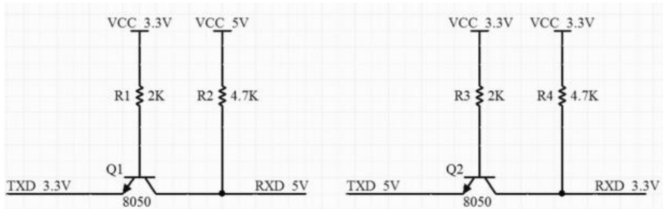
Figure 10 Level-Shifting Circuit
