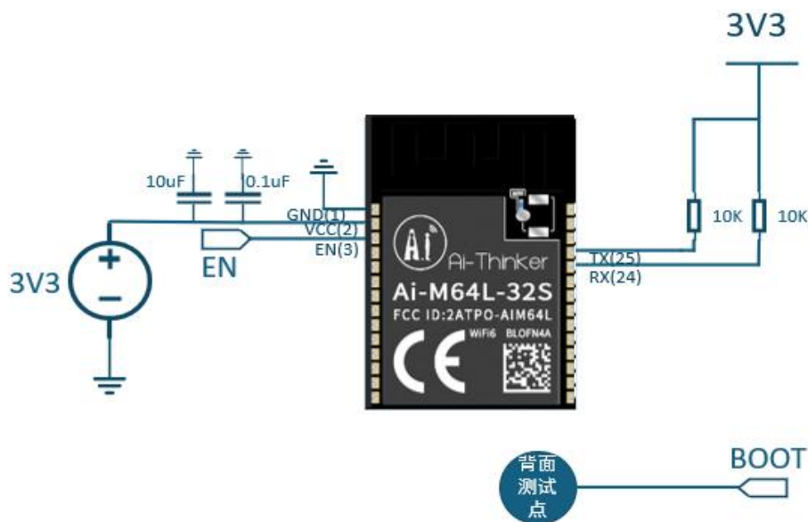
Figure 10 Application Reference Circuit
