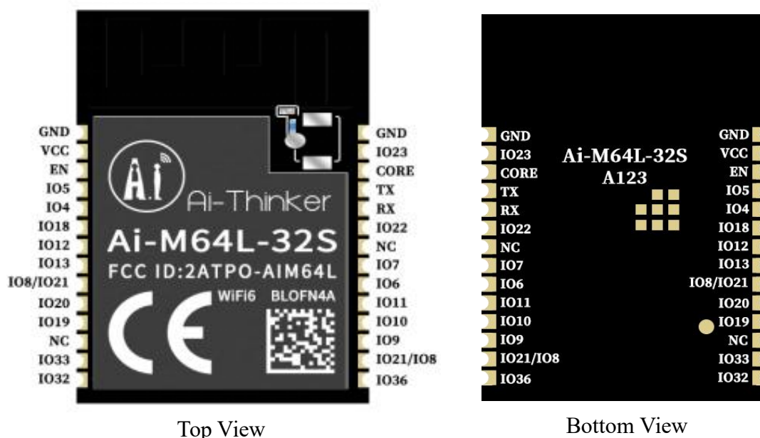
Figure 5 Pin Diagram
