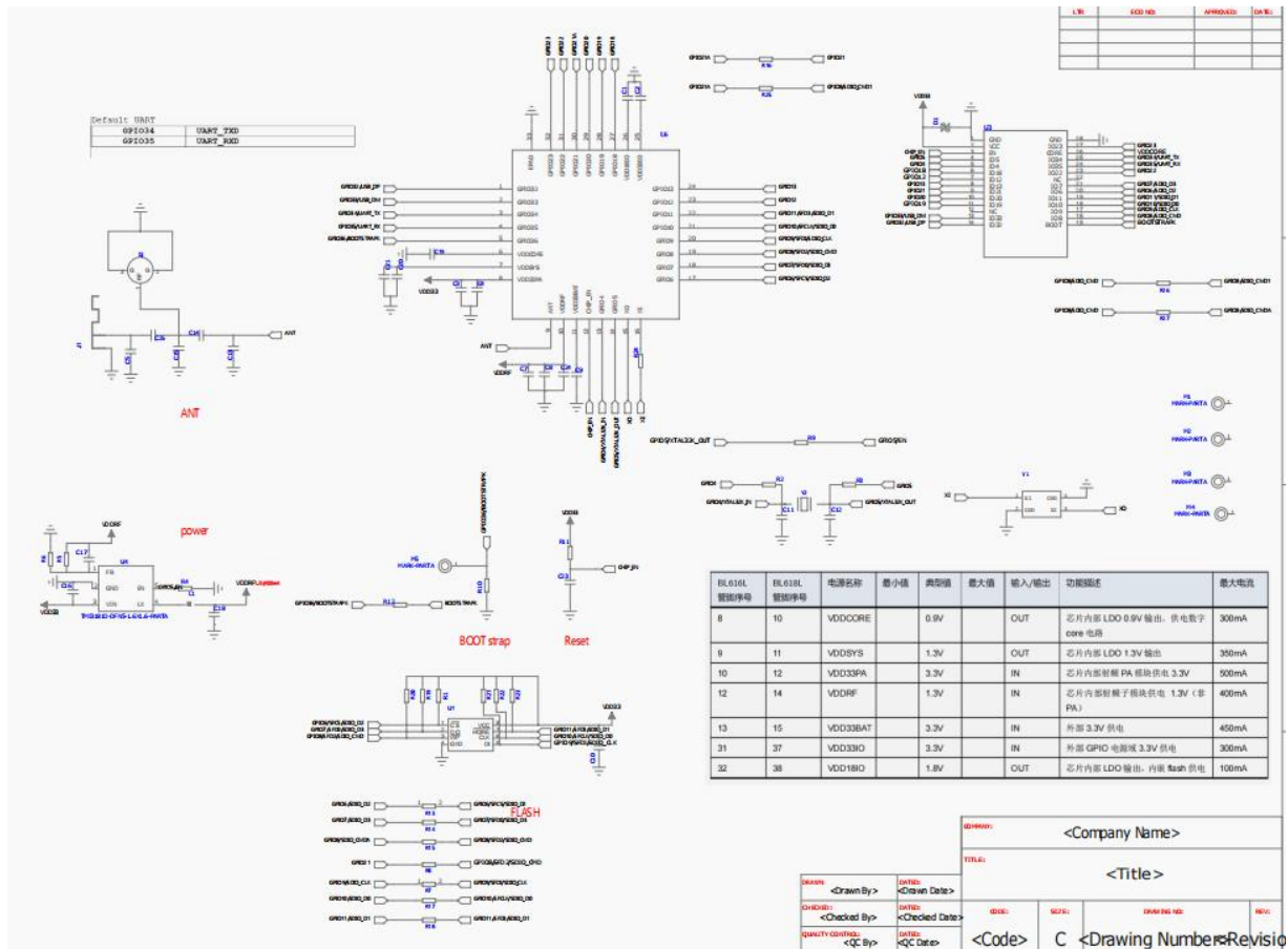
Figure 6 Schematic
