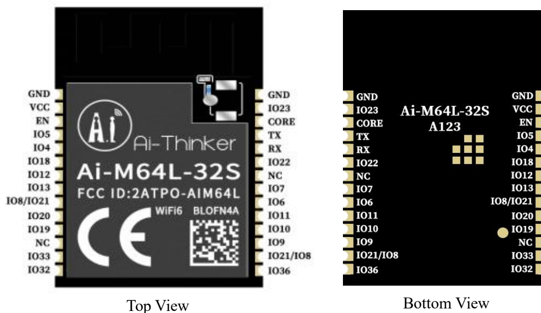
Figure 5 Pin Diagram
