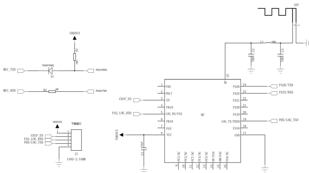
Figure 8 Application Reference Circuit
