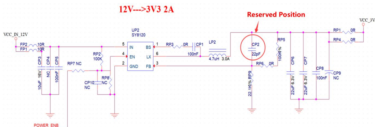
Figure 10 DC-DC Buck Circuit
