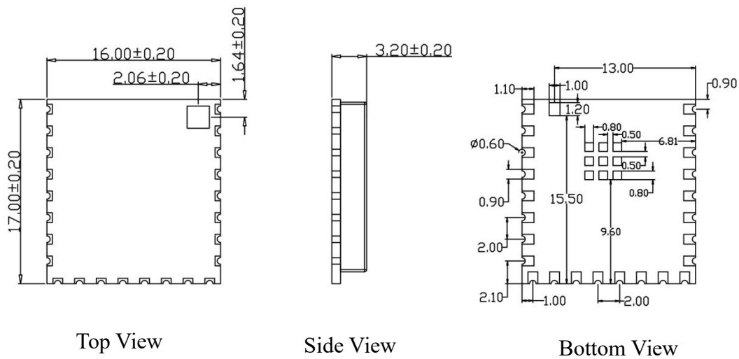
Figure 3 Module Dimensions (Unit: mm)
