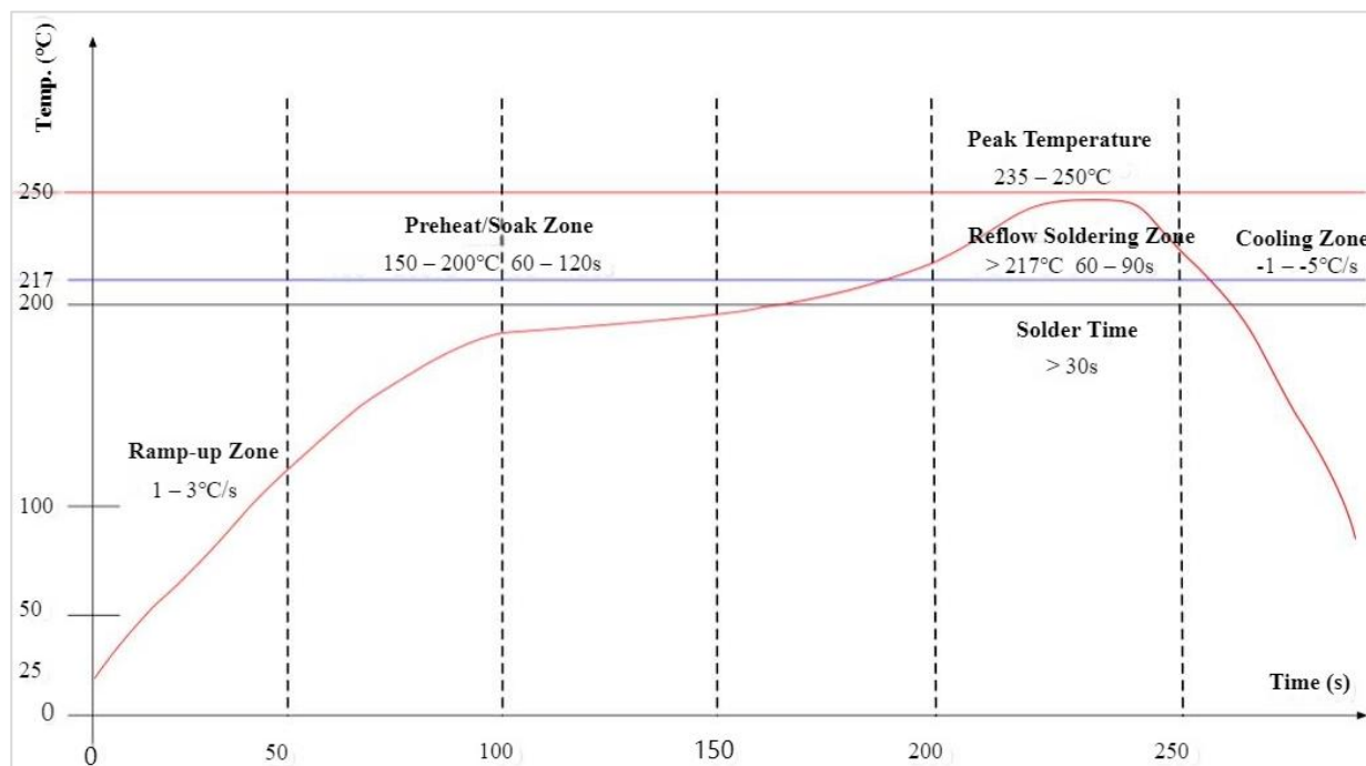
Figure 12 Reflow Soldering Profile
