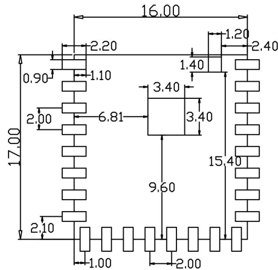
Figure 9 Recommended PCB Footprint Dimensions (Unit: mm)
