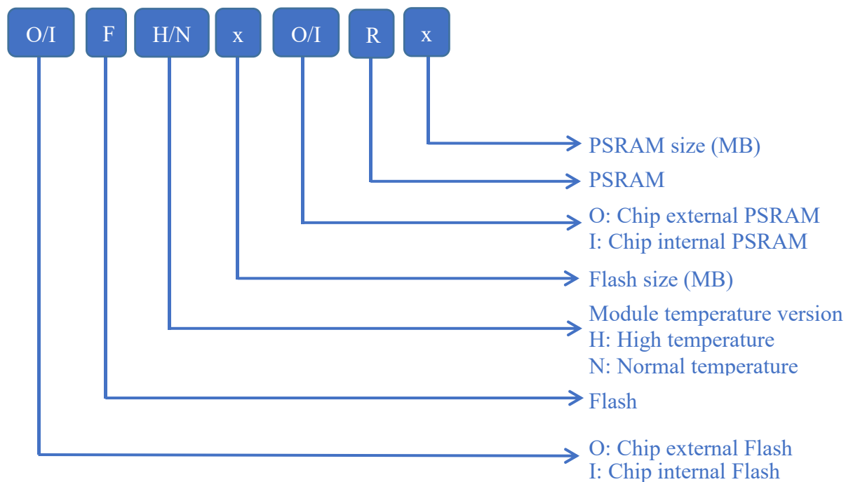
Figure 4 Shield Cover Marking Information
