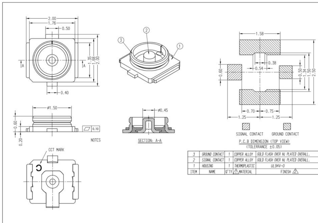
Figure 5 External Antenna Connector Dimensions (Unit: mm)
