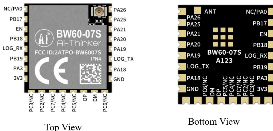
Figure 6 Pin Diagram
