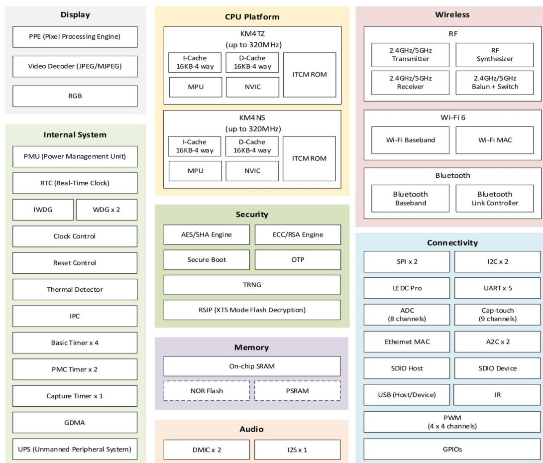
Figure 1 Main Chip Architecture Diagram
