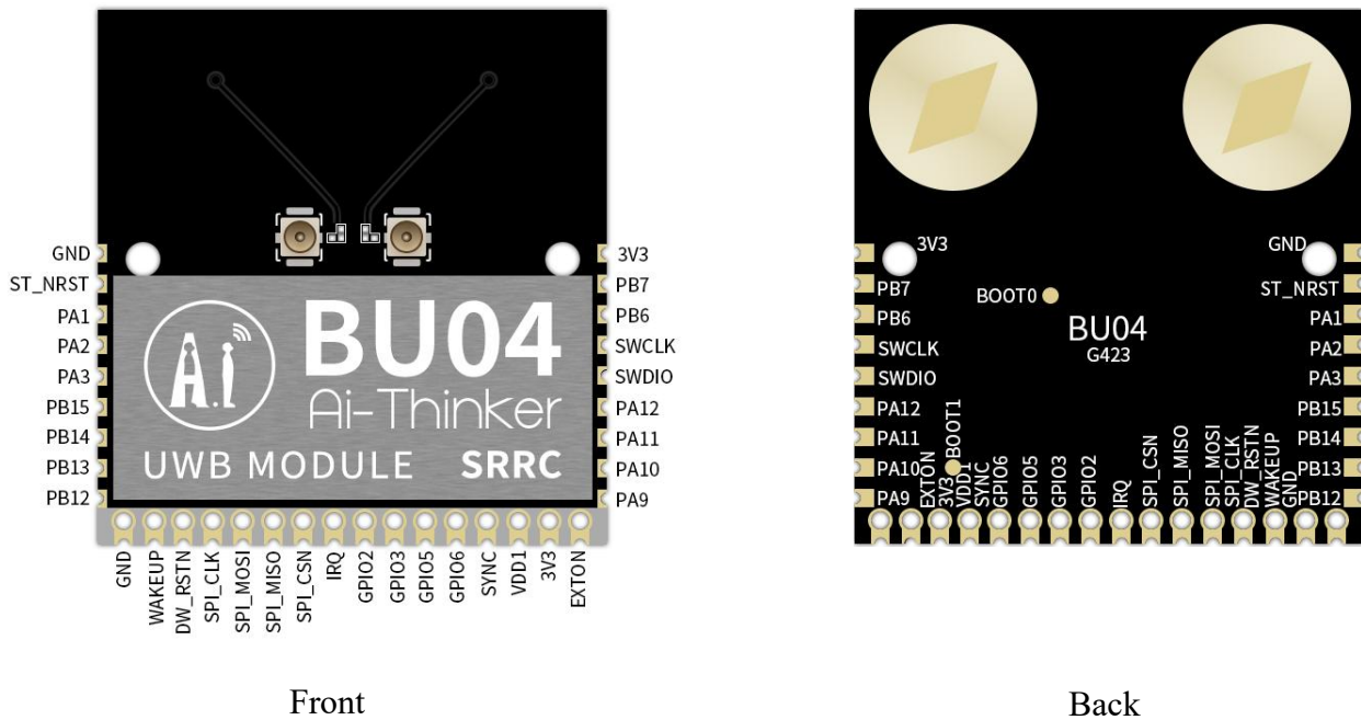
Figure 5 Pin diagram
