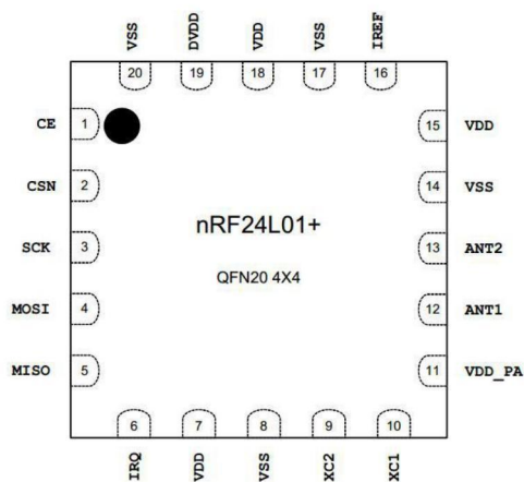
Chip Appearance Diagram
