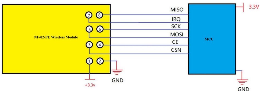
Connection Diagram between MCU and NF-02-PE
