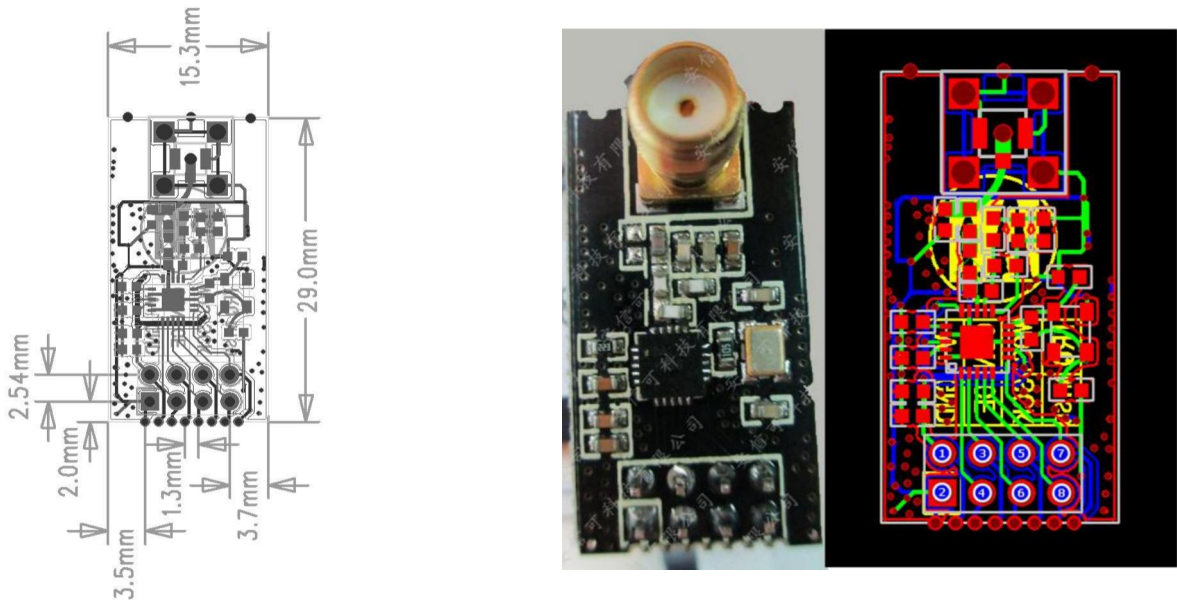
Chip Appearance Diagram
