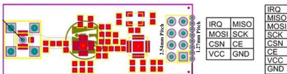
Pin Definition Diagram
