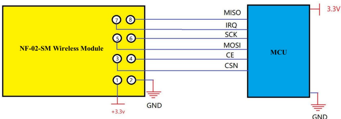
Connection Diagram between MCU and NF-02-SM
