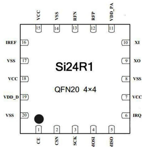
Chip Appearance Diagram
