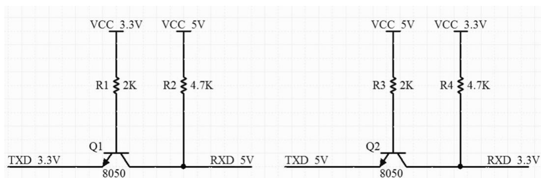
Figure 15 Level Shift Circuit
