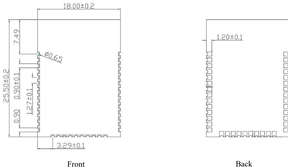
Figure 4 dimension diagram
