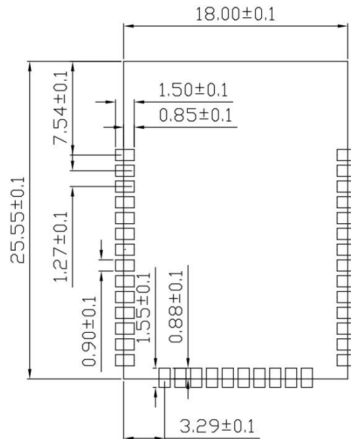
Figure 12 Recommended PCB Package Size
