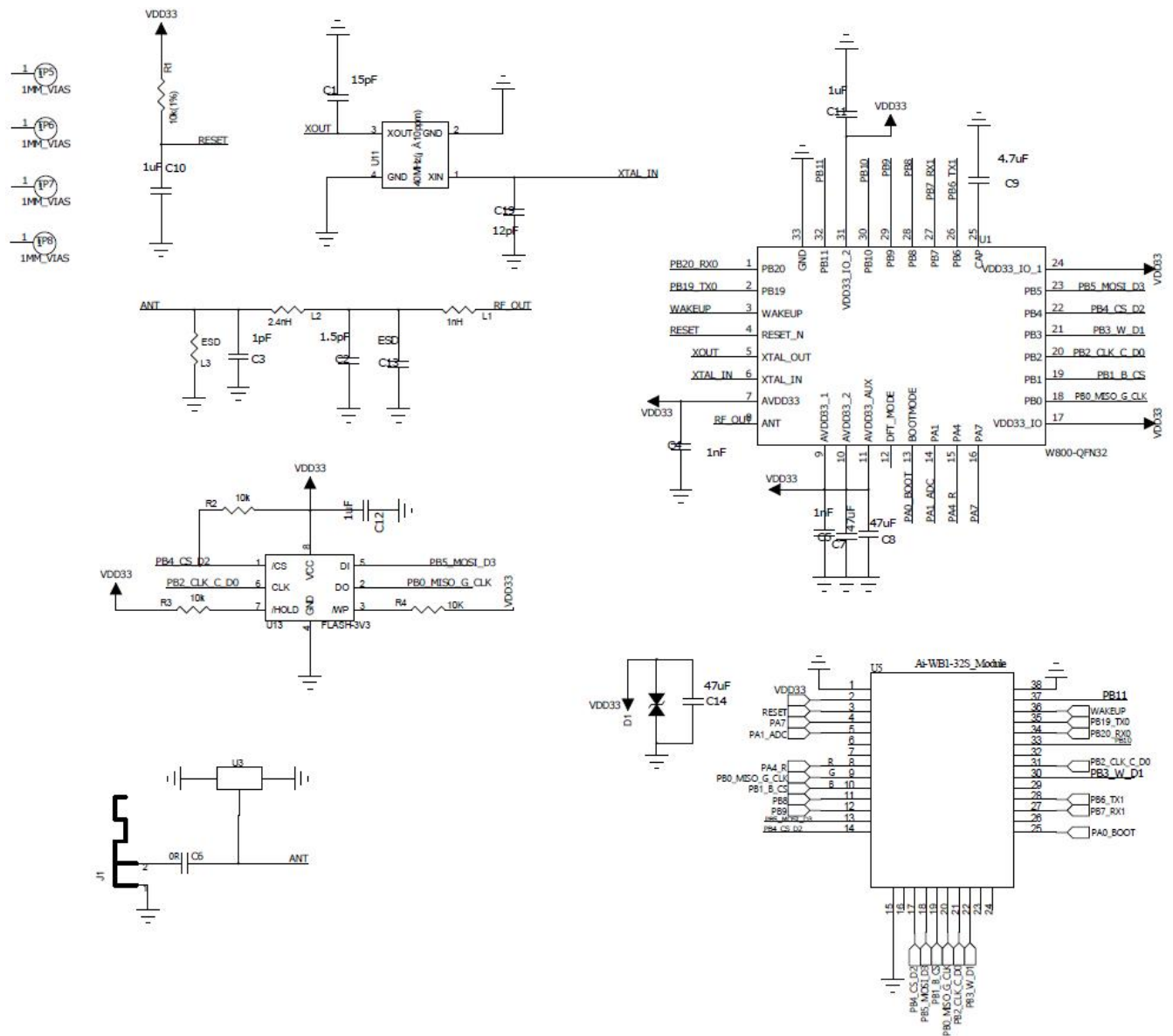
Figure 6 Schematic
