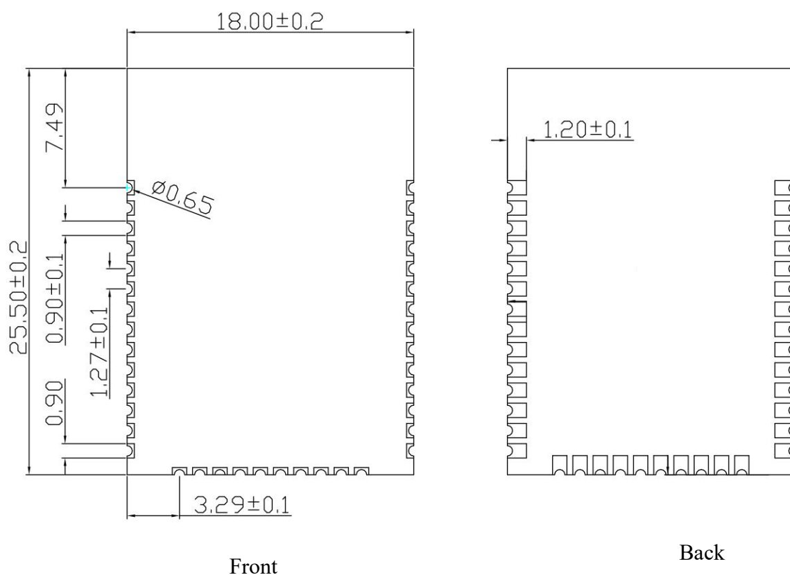
Figure 4 Dimension diagram
