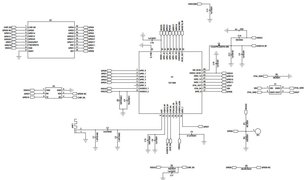
Figure 7 Module schematic
