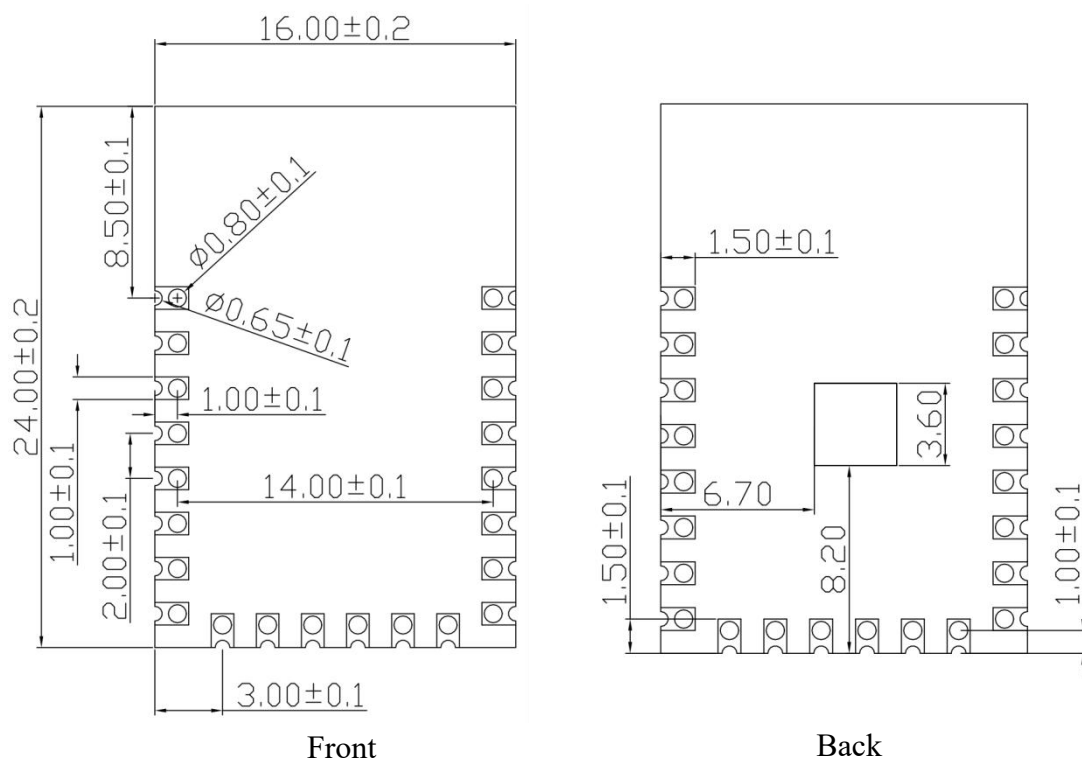
Figure 4 Dimension diagram
