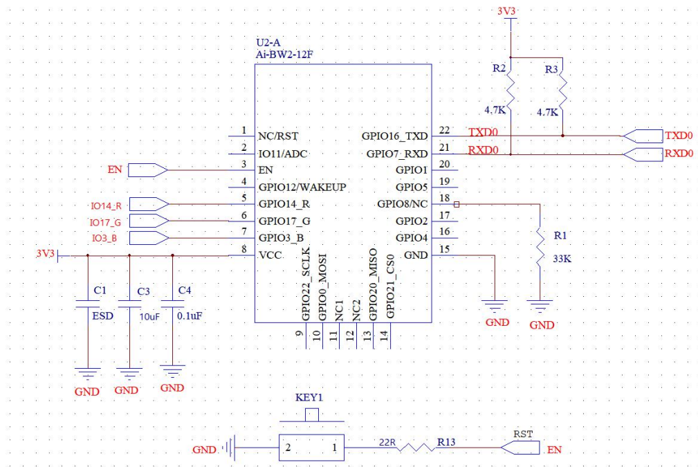
Figure 11 Application circuit diagram
