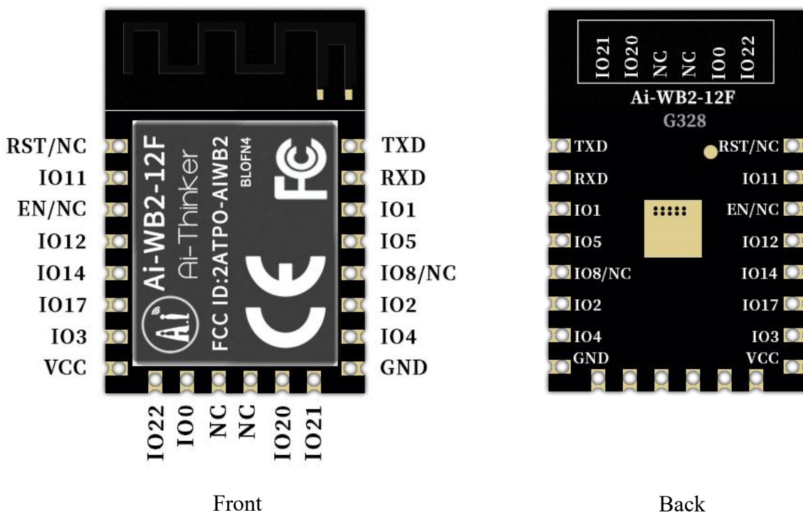
Figure 6 Schematic diagram of module pins
