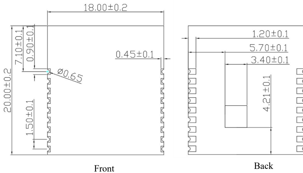
Figure 4 Dimension diagram
