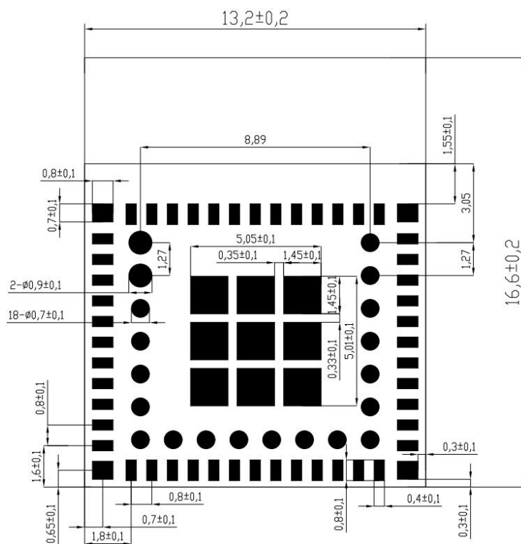
Figure 4 Dimension diagram
