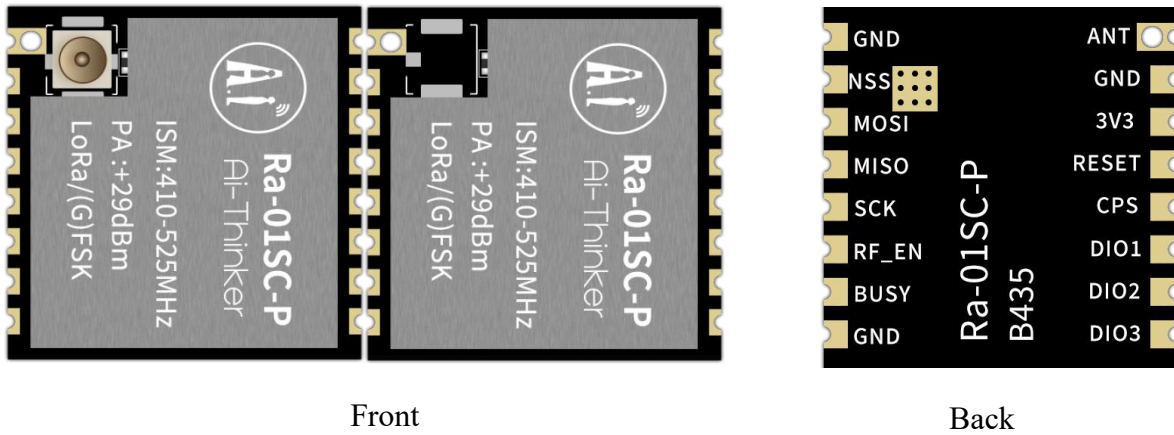
Figure 3 Appearance(rendering is for reference only, the actual object shall prevail)
