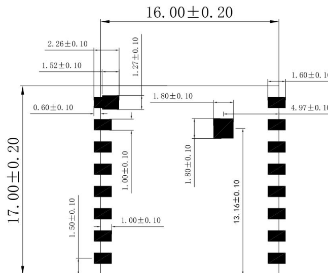
Figure 9 Recommended PCB package dimensions (unit: mm)
