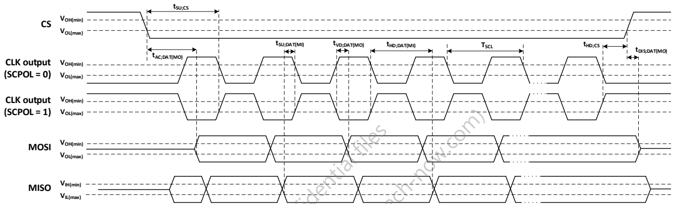
Figure 9-11 Timing diagram for master (SCPH = 1)
