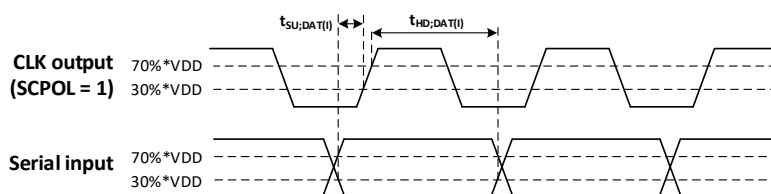
Figure 9-8 Input timing diagram (SCPH = 1)
