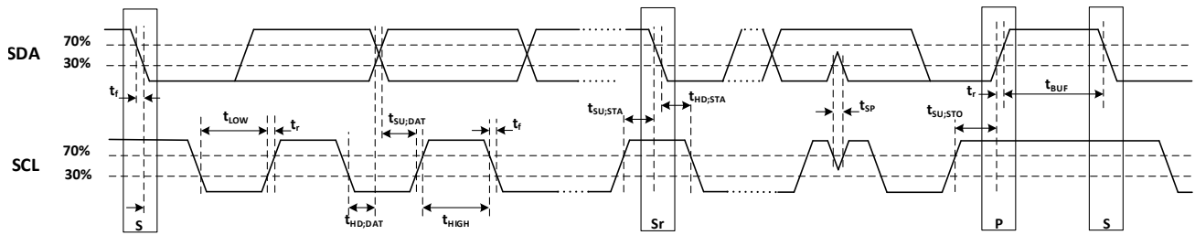
Figure 9-14 Timing diagram of I2C (FS/SS mode)
