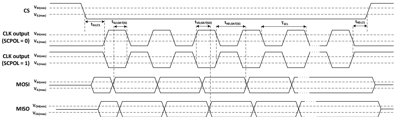
Figure 9-13 Timing diagram for slave (SCPH = 1)
