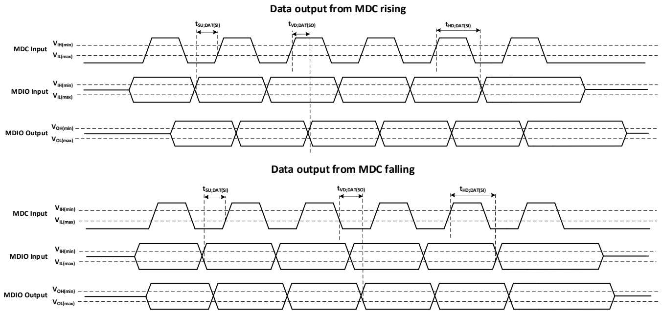
Figure 9-27 Timing parameters for MDC/MDIO in slave mode
