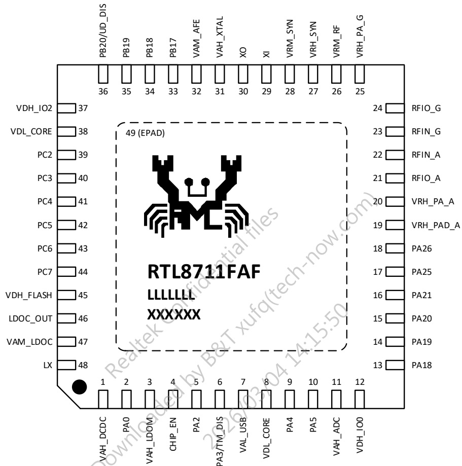
Figure 5-1 RTL8711FAF series pinout
