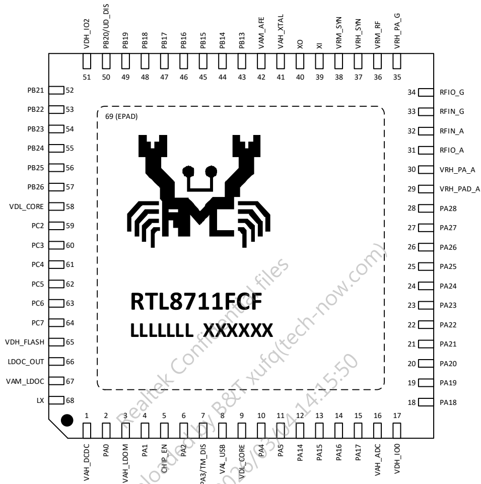
Figure 5-2 RTL8711FCF series pinout
