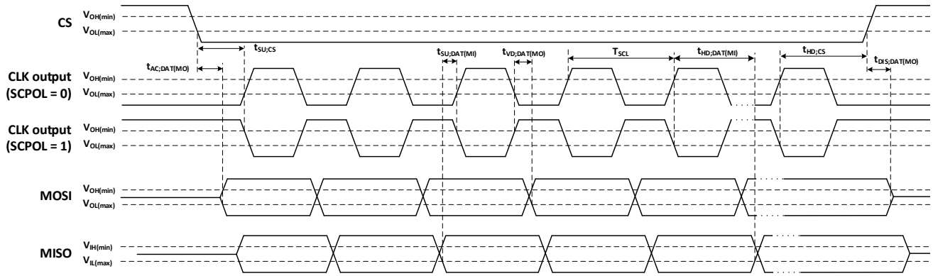
Figure 9-10 Timing diagram for master (SCPH = 0)
