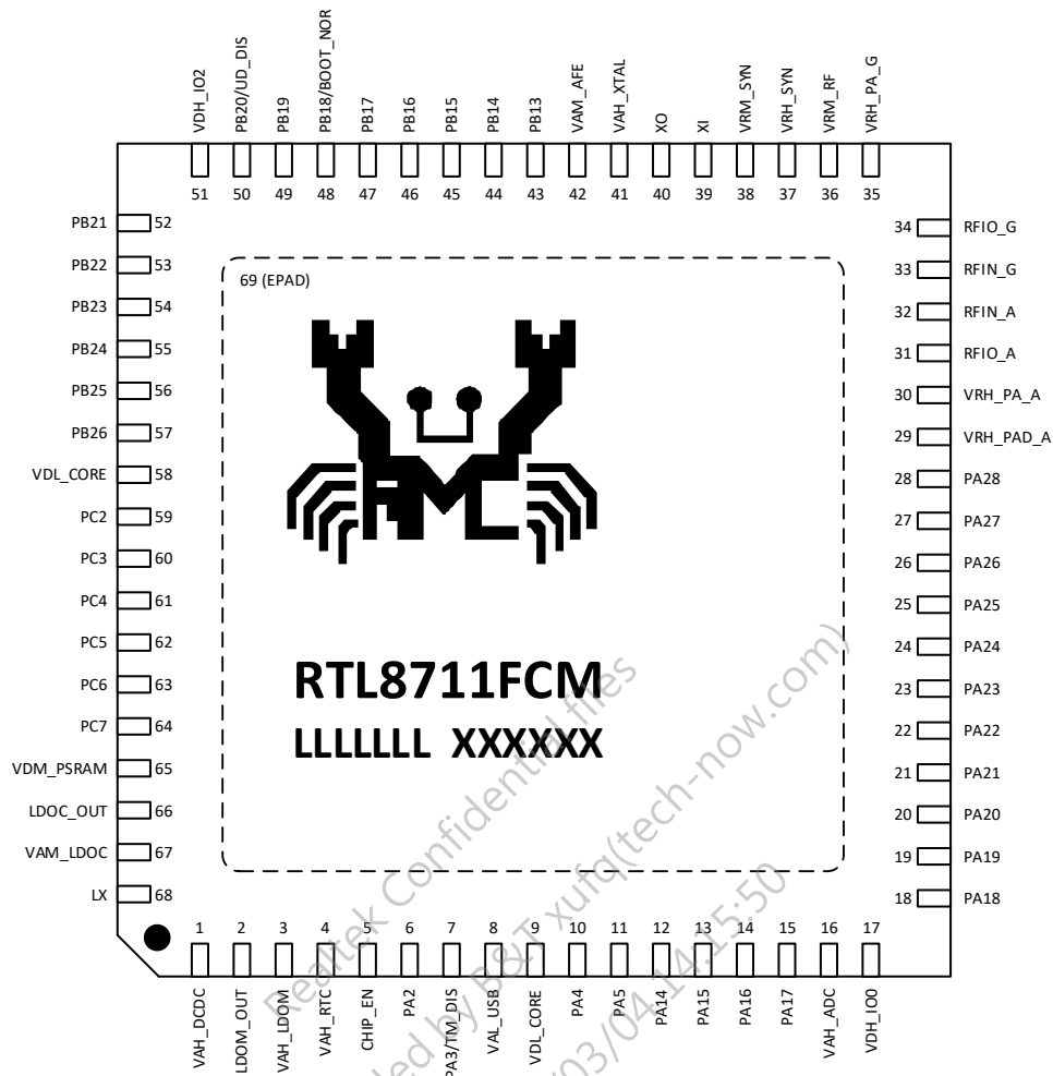
Figure 5-3 RTL8711FCM series pinout
