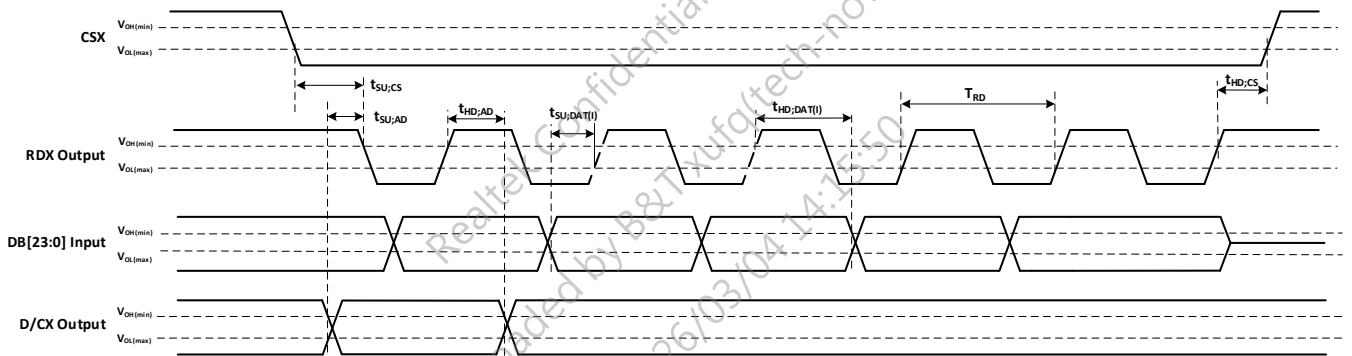
Figure 9-30 Read timing parameters for LCDC in MCU mode
