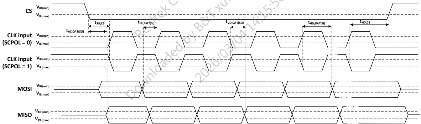
Figure 9-12 Timing diagram for slave (SCPH = 0)
