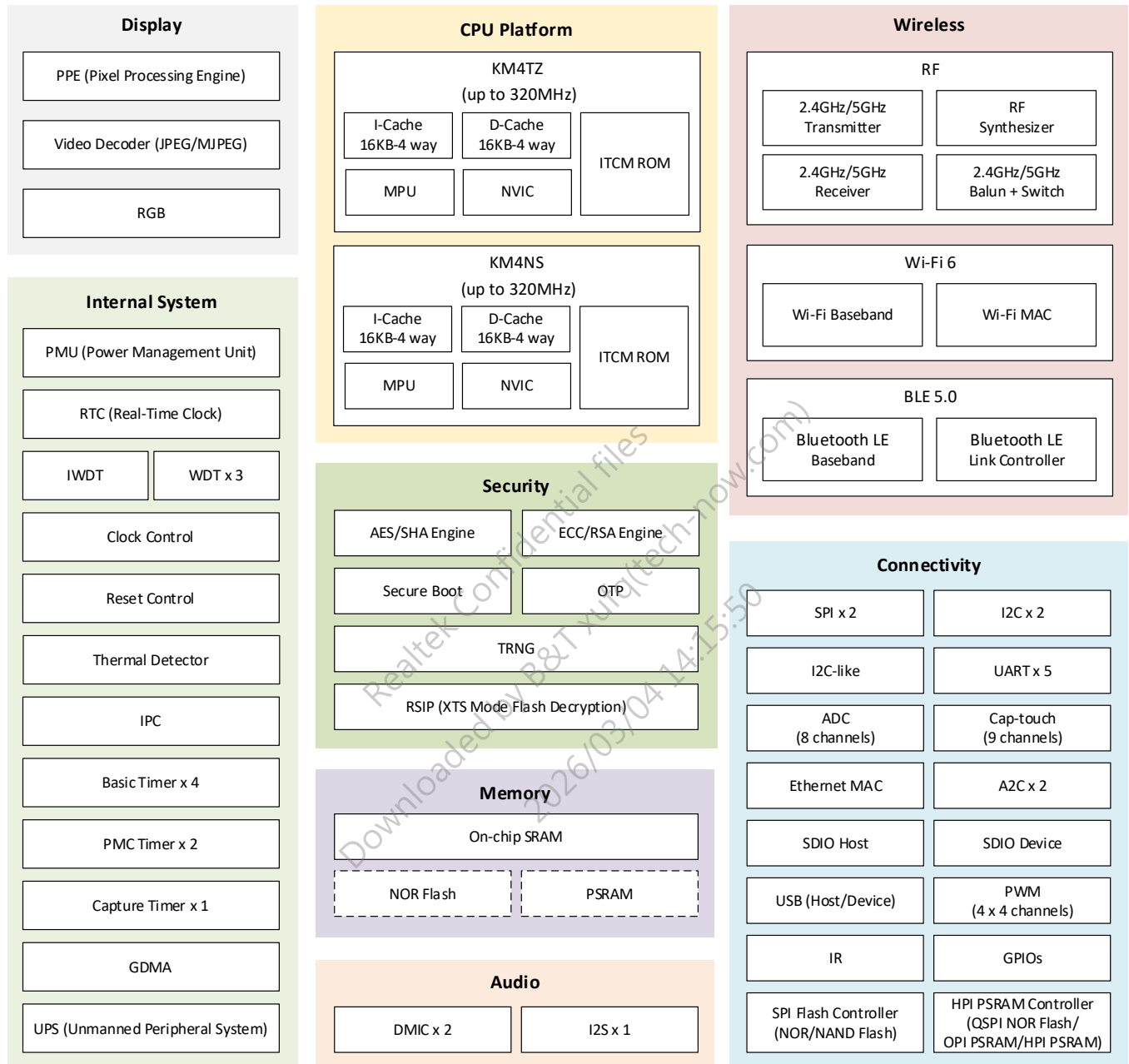
Figure 4-1 Block diagram
