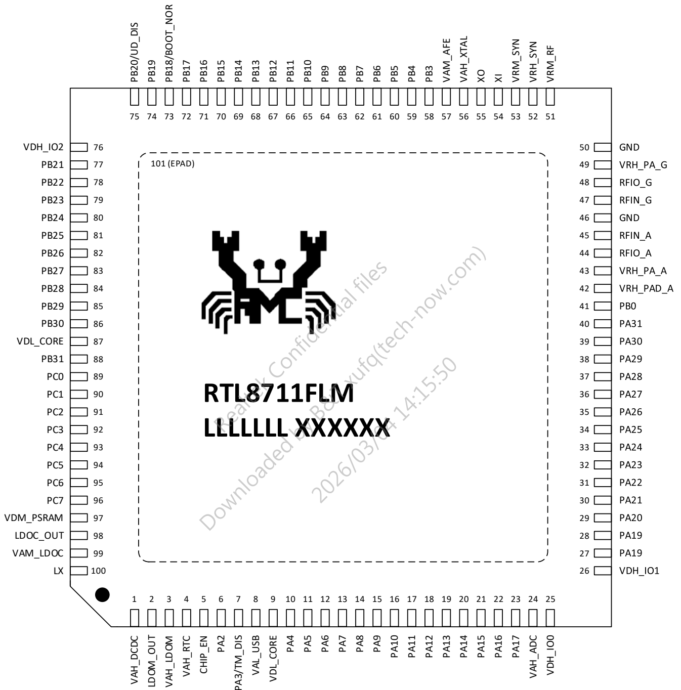
Figure 5-4 RTL8711FLM series pinout
