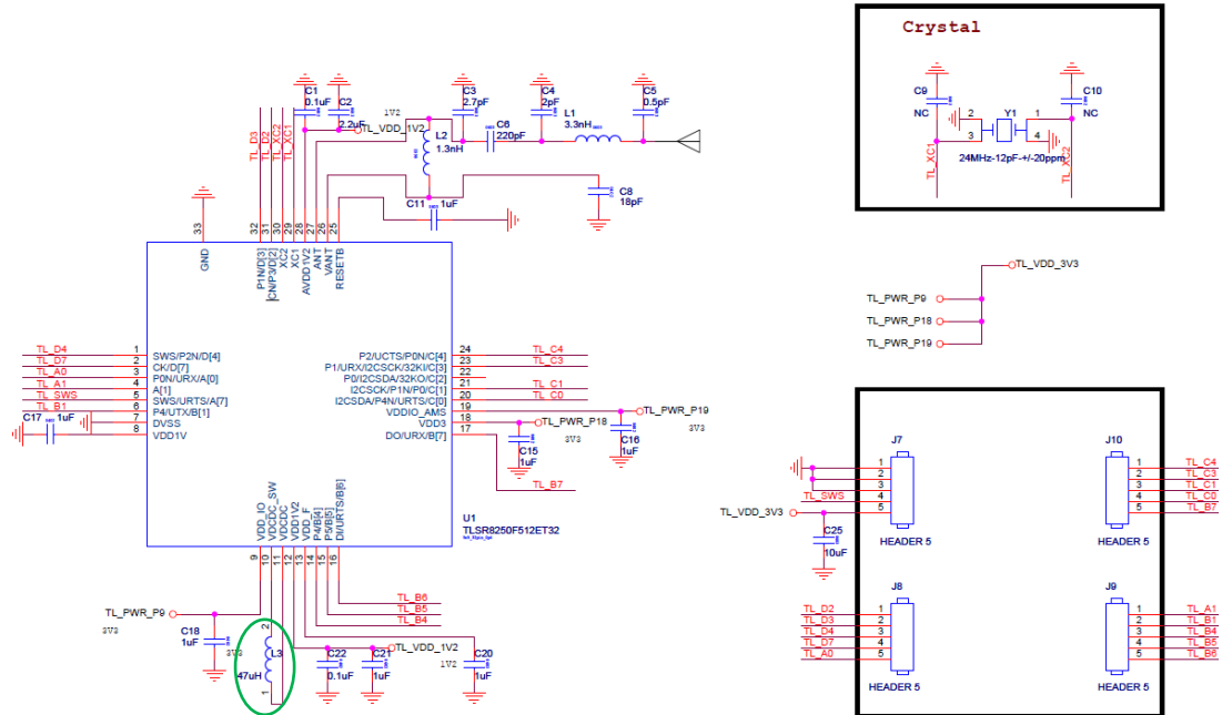
Figure 17- 1 Schematic for TLSR8250F512ET32
