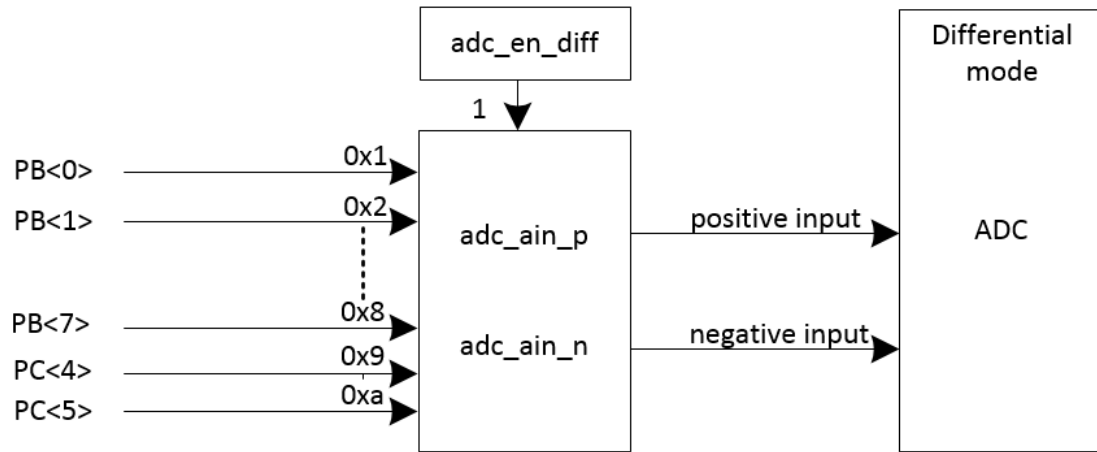
Figure 9- 1 Block diagram of ADC
