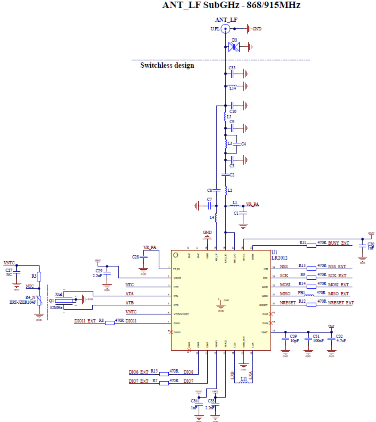
Figure 23-2: LR2012 Reference Design Schematic
