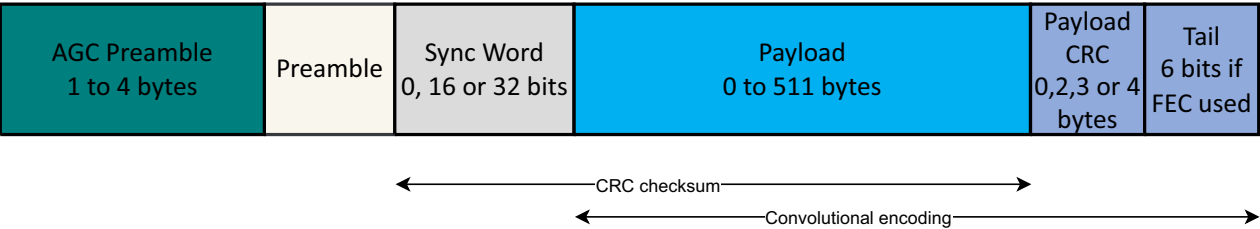
Figure 18-1: FLRC Fixed-length Packet Format
