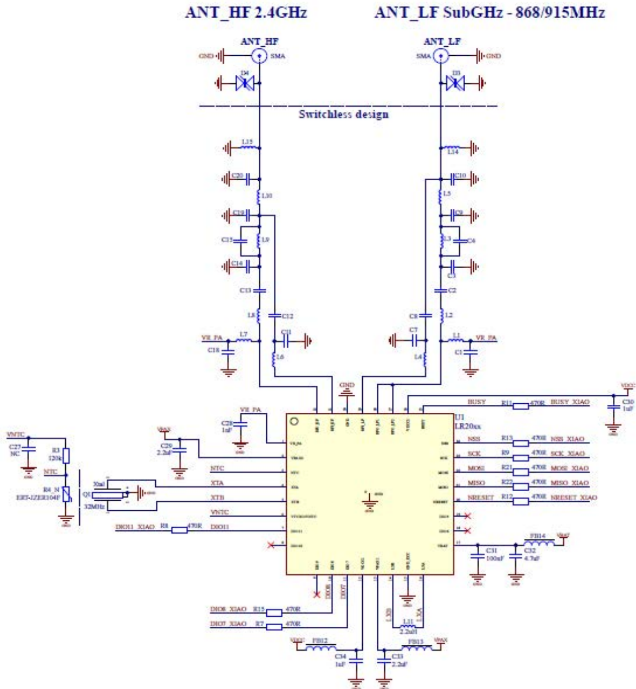
Figure 23-1: LR2021/LR2022 Reference Design Schematic
