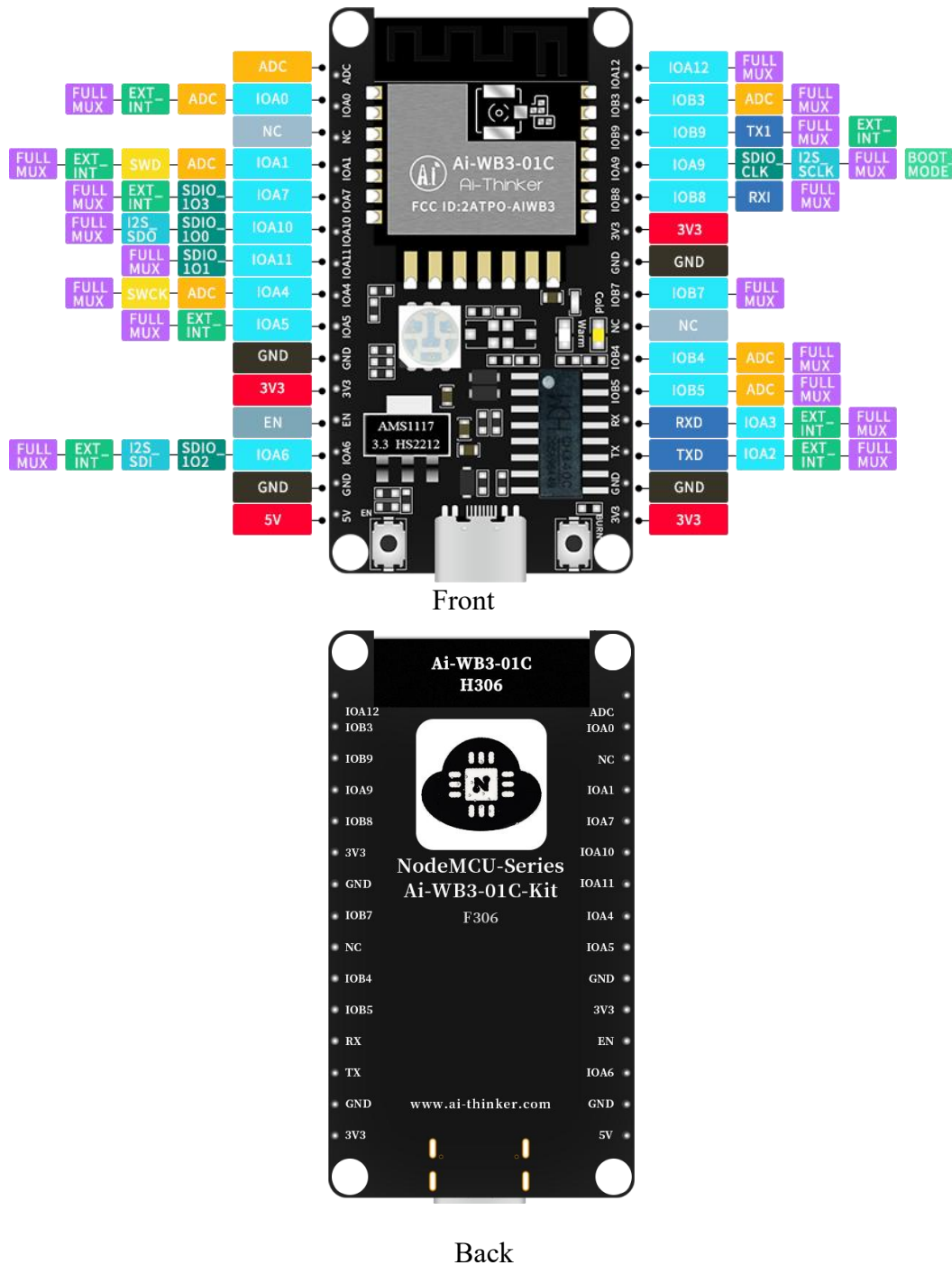
Figure 6 pin diagram
