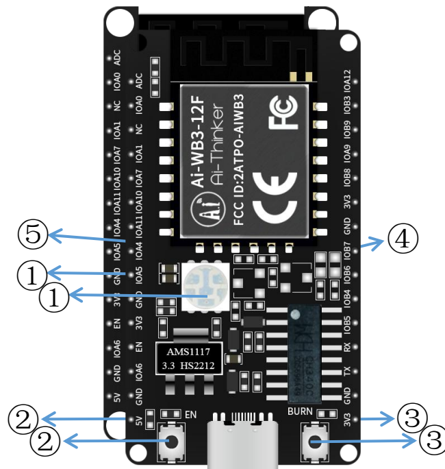
Figure 5 Ai-WB3-01C-Kit indicator light and key position
